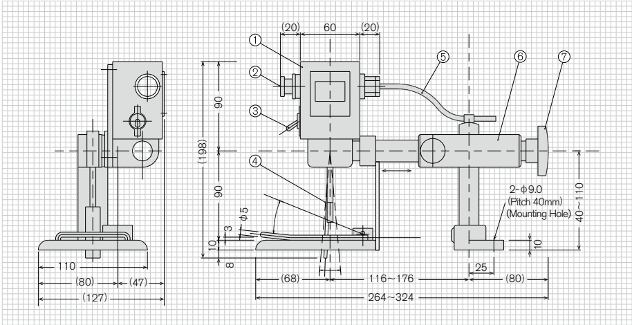
① Body (MF-6C) ② Dead band adjustment handle ③ Power switch ON/OFF ④ Feeler lever ⑤ Connection cord ⑥ Holder ⑦ Adjustment handle (Left/Right)
